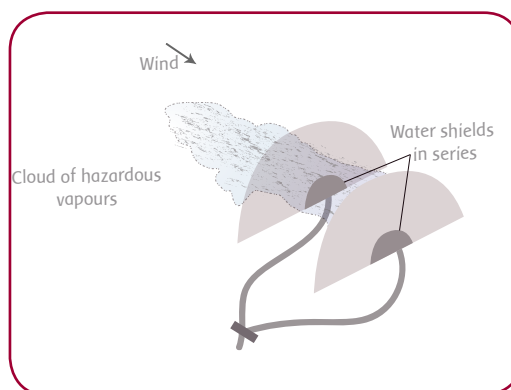
Water curtain sprayed by water shields in series.
