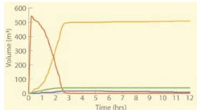
Spill involving 500 tonnes of styrene at a rate of 3,000 tonnes/hour for 10 minutes Wind 10 m/s
