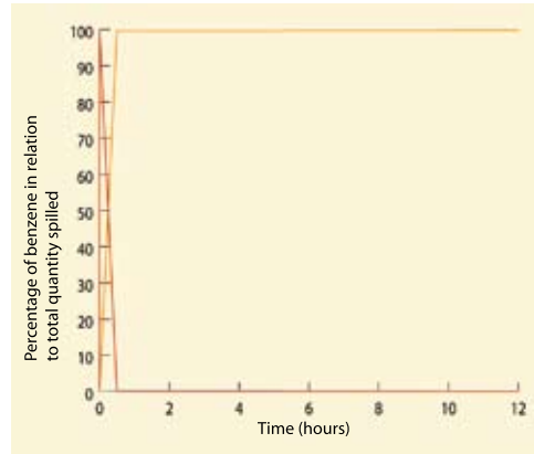
Instantaneous spillage of 500 tonnes of benzene. Wind speed: 10 m/s
